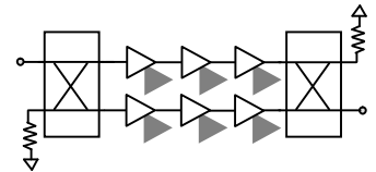
3-stage Balanced Type
